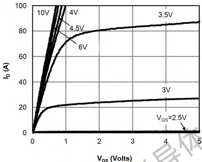
Figure 1: On-Region Characteristics
